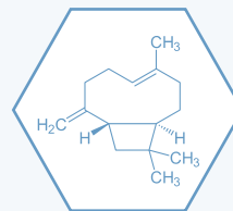
B-Caryophyllene
