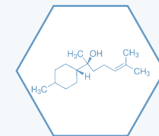
α-Bisabolol
