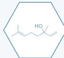
Linalool
