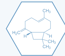
Caryophyllene
