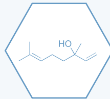
Linalool
