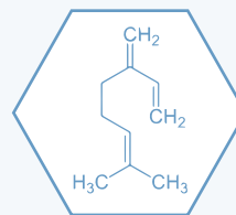
Myrcene
