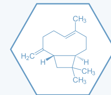
Caryophyllene
