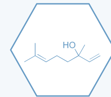
Linalool
