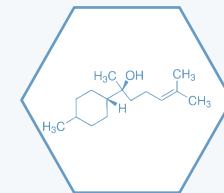
α-Bisabolol
