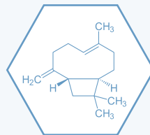
B-Caryophyllene
