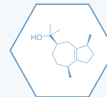
(-)-Guaioil
