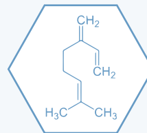
Myrcene
